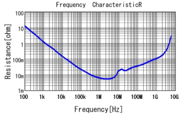
■ GRM188C71C225KE11 R DCOV, 25degC
