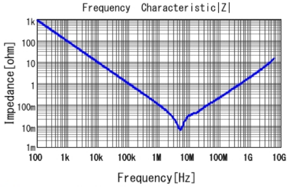
■ GRM188C71C225KE11 |Z| DCOV, 25degC
