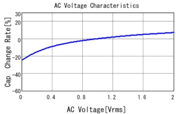
■ GRM188C71C225KE11 C-AC Voltage capchange, DCOV, 25.0d
