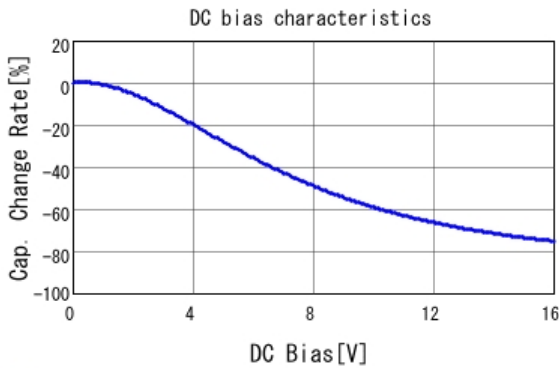
■ GRM188C71C225KE11 C-DC bias capchange, 25.0degC, AC1V
