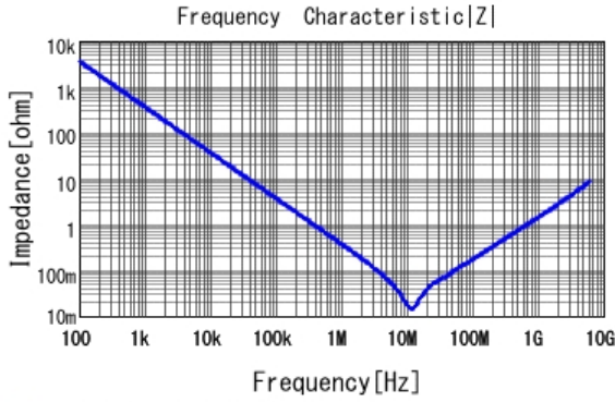
■ GRM155C80J474KE19 |Z| DCOV, 25degC
