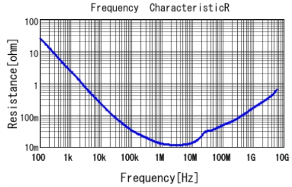
■ GRM155C80J474KE19 R DCOV, 25degC
