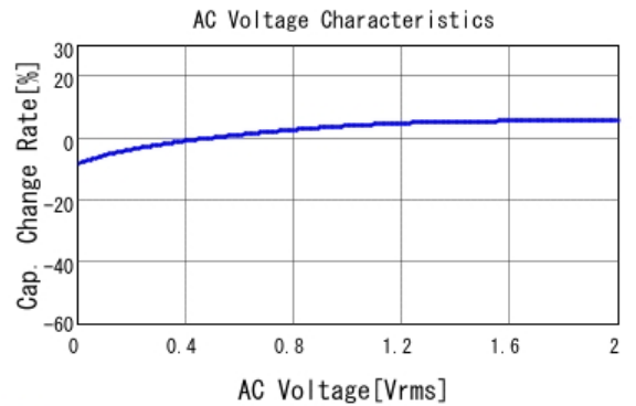
■ GRM155C80J474KE19 C-AC Voltage capchange, DCOV, 25.0d
