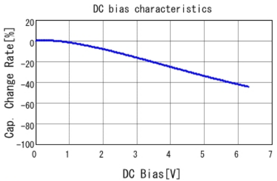
■ GRM155C80J474KE19 C-DC bias capchange, 25.0degC, ACO.
