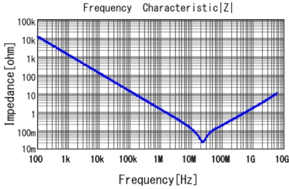
■ GRM155C8YA224KE01 |Z| DCOV, 25degC
