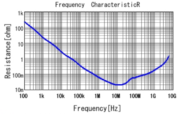
■ GRM155C8YA224KE01 R DCOV, 25degC
