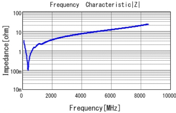
■ GRM1555C1H471GA01 |Z| DCOV, 25degC
