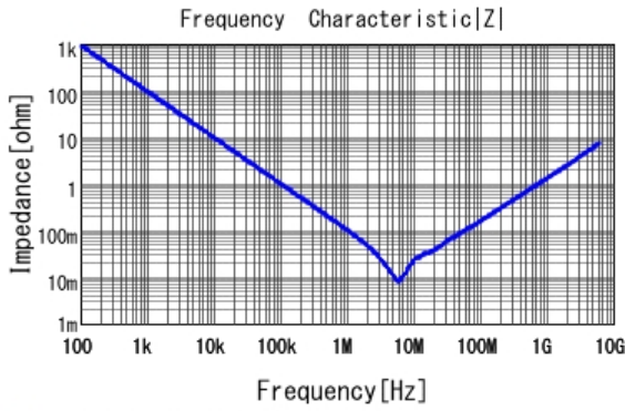
■ GRM155C81C225KE11 |Z| DCOV, 25degC
