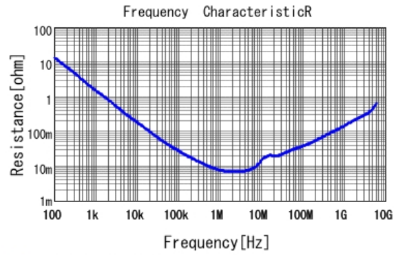
■ GRM155C81C225KE11 R DCOV, 25degC
