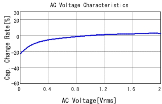
■ GRM155C81C225KE11 C-AC Voltage capchange, DCOV, 25.0d
