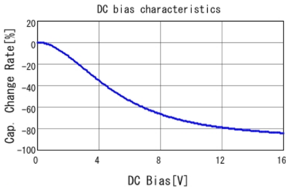
■ GRM155C81C225KE11 C-DC bias capchange, 25.0degC, AC1V
