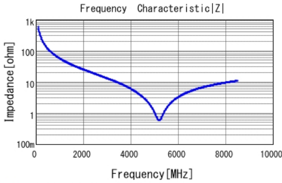
■ GCM1555C1H2R7CA16 |Z| DC0V, 25degC
