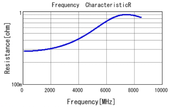
■ GCM1555C1H2R7CA16 R DC0V, 25degC
