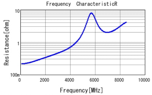
■ GCM1555C1H9R0BA16 R DCOV, 25degC
