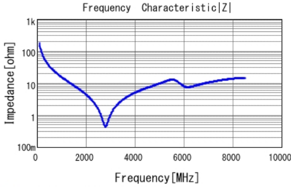
■ GCM1555C1H9R0BA16 |Z| DCOV, 25degC
