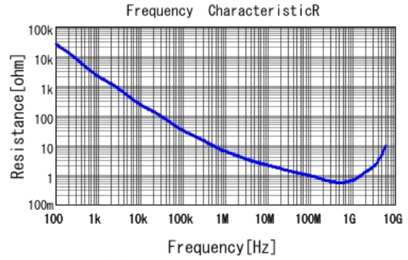
GCM155R71H331KA37 R DCOV, 25degC
