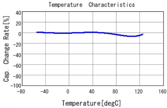
■ GCM155R71H331KA37 C-Temp. capchange, DC0.0V, AC1.0V rm
