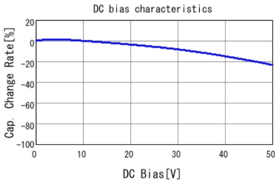
GCM155R71H331KA37 C-DC bias capchange, 25.0degC, AC1.
