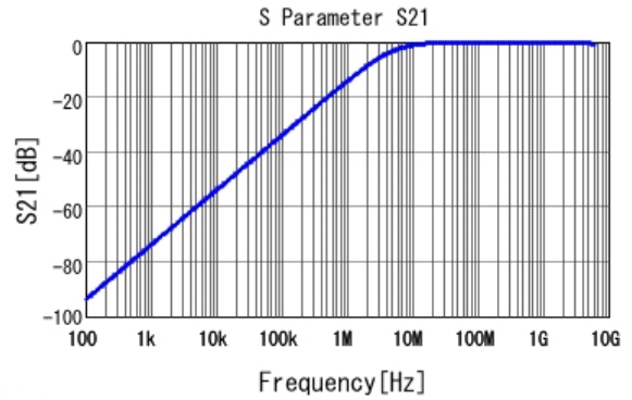
■ GCM155R71H331KA37 S21 DC0V, 25degC
