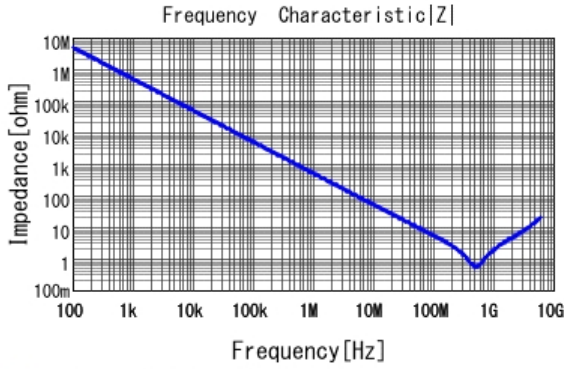
GCM155R71H331KA37 |Z| DCOV, 25degC
