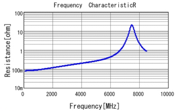
■ GJM1555C1H9R1DB01 R DCOV, 25degC
