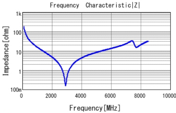
■ GJM1555C1H9R1DB01 |Z| DCOV, 25degC
