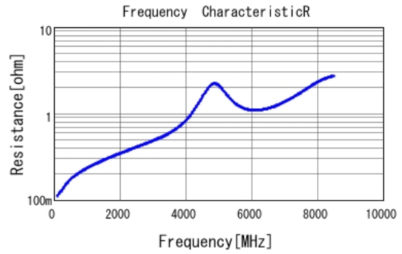
■ GCM1555C1H150JA16 R DCOV, 25degC
