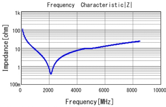
■ GCM1555C1H150JA16 |Z| DCOV, 25degC
