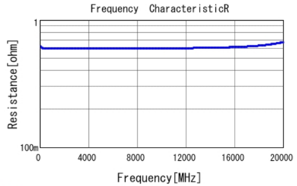
GJM1555C1HR10BB01 R DCOV, 25degC
