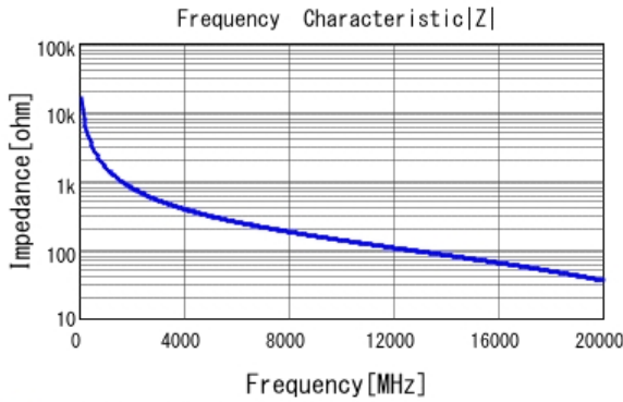
GJM1555C1HR10BB01 |Z| DCOV, 25degC
