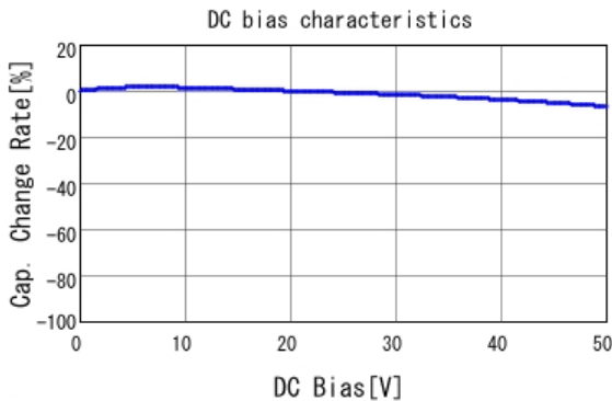
■ GCJ188R71H102KA01 C-DC bias capchange, 25.0degC, AC1.
