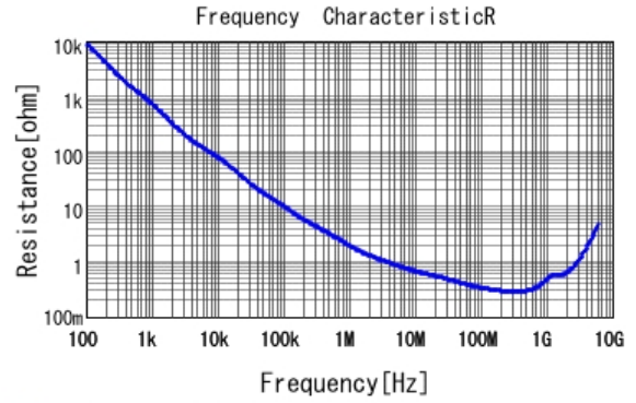
GCM155R72A102KA37 R DCOV, 25degC
