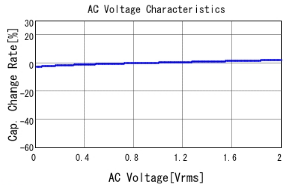
GCM155R72A102KA37 C-AC Voltage capchange, DCOV, 25.0d
