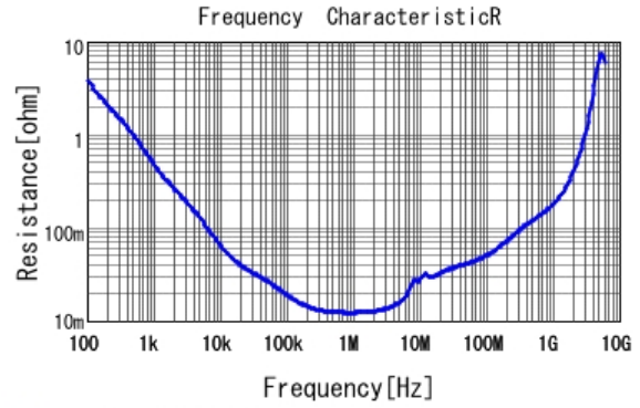
■ GCJ21BR71A225KA01 R DC0V, 25degC
