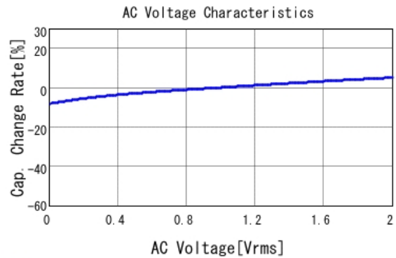
■ GCJ21BR71A225KA01 C-AC Voltage capchange, DC0V, 25.0d
