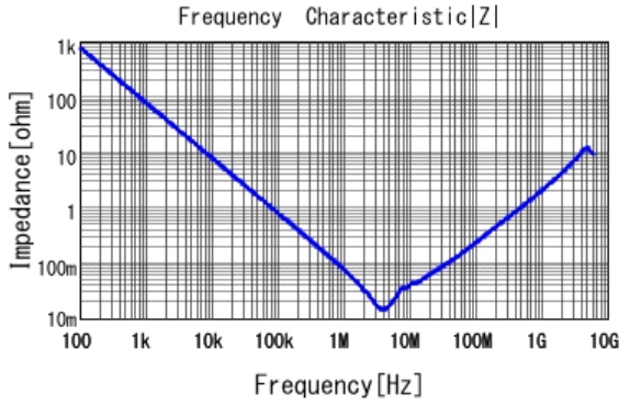
■ GCJ21BR71A225KA01 |Z| DC0V, 25degC
