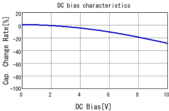
■ GCJ21BR71A225KA01 C-DC bias capchange, 25.0degC, AC1.
