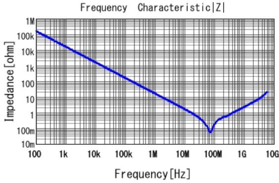
■ GCD188R72A103KA01 |Z| DCOV, 25degC
