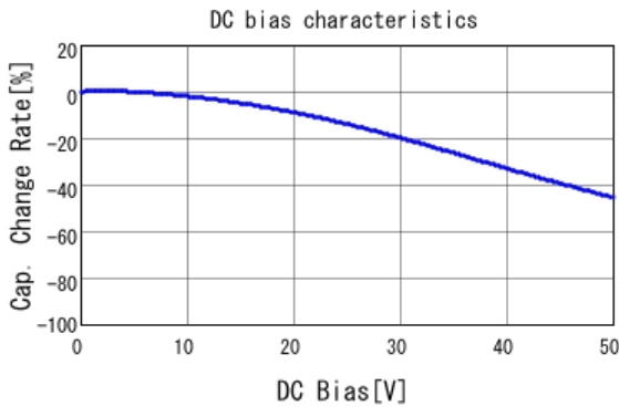
GCM155R71H103KA55 C-DC bias capchange, 25.0degC, AC1.
