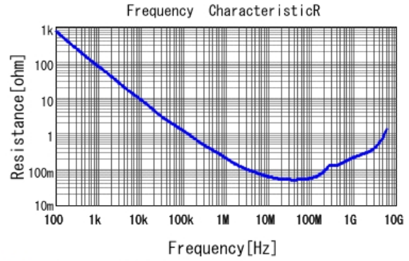
GCM155R71H103KA55 R DCOV, 25degC
