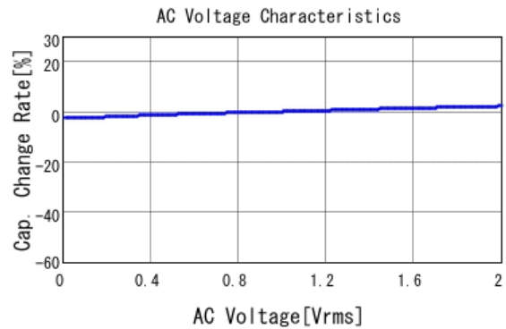
GCM155R71H103KA55 C-AC Voltage capchange, DCOV, 25.0d
