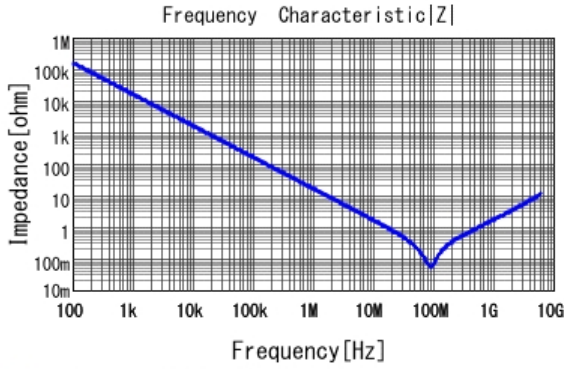
GCM155R71H103KA55 |Z| DCOV, 25degC
