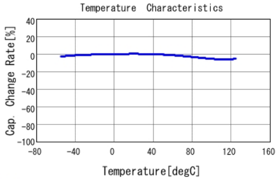
■ GCM155R71H103KA55 C-Temp. capchange, DC0.0V, AC1.0V rm
