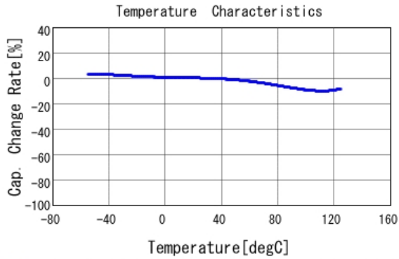
■ GCM155R71E682KA37 C-Temp. capchange, DC0.0V, AC1.0V rm
