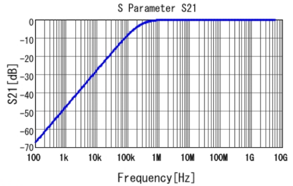
■ GCM155R71E682KA37 S21 DC0V, 25degC
