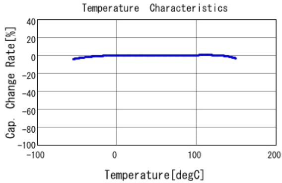
■ GCJ188R92A153KA01 C-Temp. capchange, DC0.0V, AC1.0Vrm
