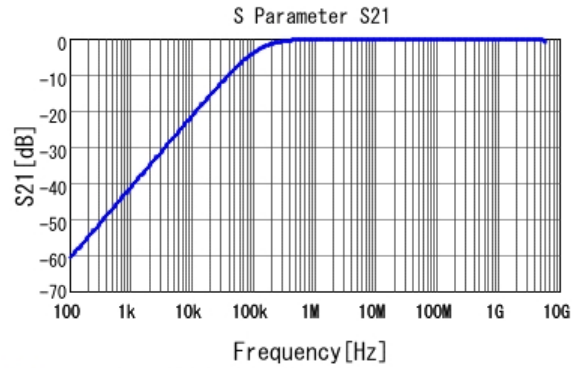
■ GCJ188R92A153KA01 S21 DC0V, 25degC
