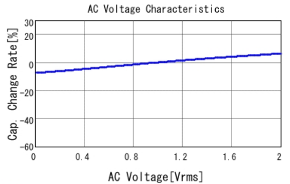
■ GCJ188R92A153KA01 C-AC Voltage capchange, DCOV, 25.0d
