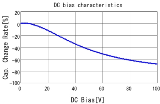
■ GCJ188R92A153KA01 C-DC bias capchange, 25.0degC, AC1.
