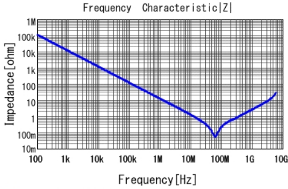
■ GCJ188R92A153KA01 |Z| DCOV, 25degC
