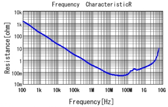
■ GCJ188R92A153KA01 R DCOV, 25degC
