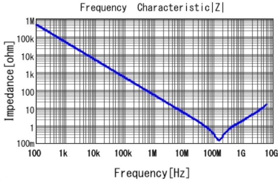
GCM155R71H332KA37 |Z| DCOV, 25degC
