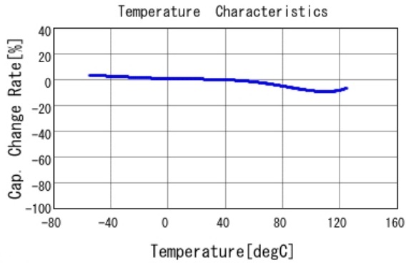
■ GCM155R71H332KA37 C-Temp. capchange, DC0.0V, AC1.0V rm
