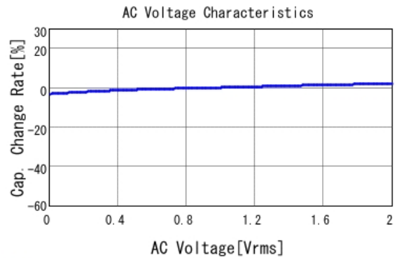
GCM155R71H332KA37 C-AC Voltage capchange, DCOV, 25.0d
