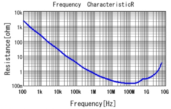
GCM155R71H332KA37 R DCOV, 25degC
