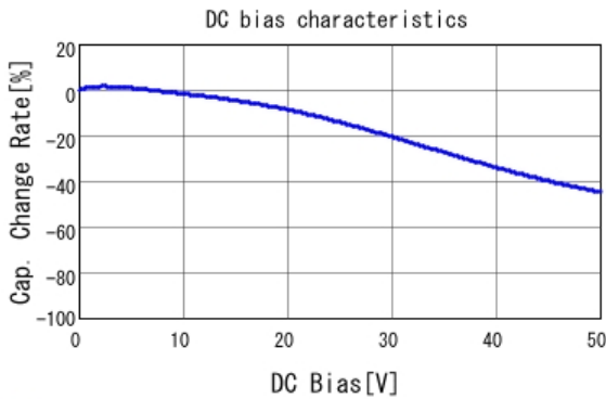
GCM155R71H332KA37 C-DC bias capchange, 25.0degC, AC1.
