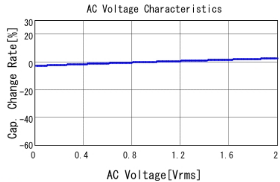
■ GCJ188R71E104KA12 C-AC Voltage capchange, DCOV, 25.0d
