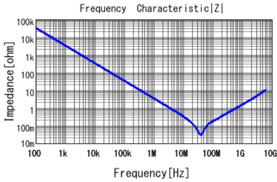
GCM155R71E473KA55 |Z| DCOV, 25degC
