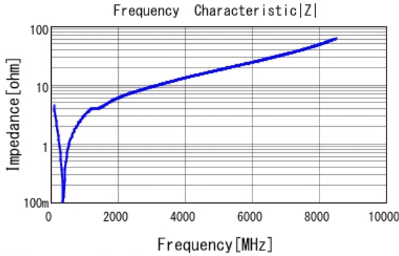
■ GCM1885C2A331JA16 |Z| DCOV, 25degC
