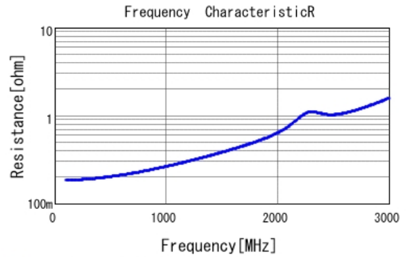
■ GRM21A5C2E560JW01 R DC0V, 25degC
