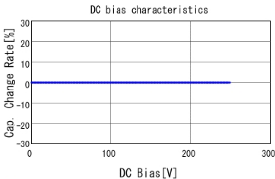
■ GRM21A5C2E560JW01 C-DC bias capchange, 25.0degC, AC1V
