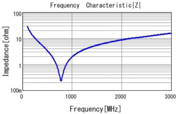
■ GRM21A5C2E560JW01 |Z| DC0V, 25degC
