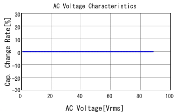
■ GRM21A5C2E560JW01 C-AC Voltage capchange, DC0V, 25.0d
