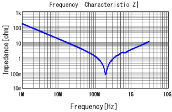
■ GRM21A7U2E102JW31 |Z| DCOV, 25degC
