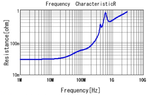
■ GRM21A7U2E102JW31 R DCOV, 25degC
