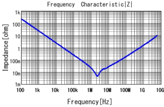
■ GRT188C81C106ME13 |Z| DCOV, 25degC
