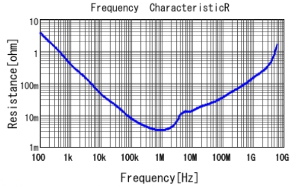
■ GRT188C81C106ME13 R DCOV, 25degC
