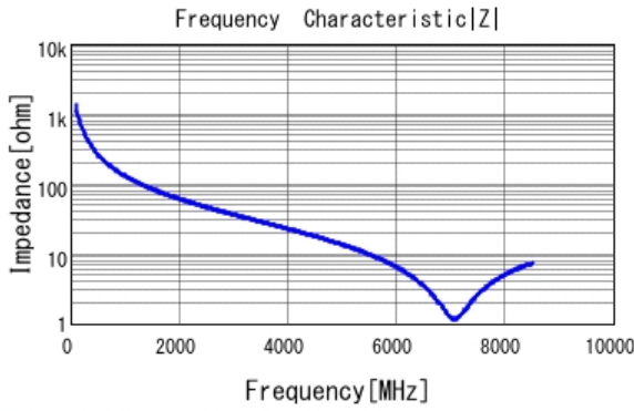
■ GCM1555C1H1R2CA16 |Z| DCOV, 25degC
