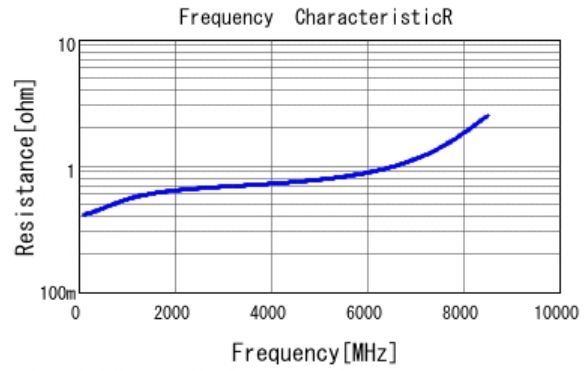
■ GCM1555C1H1R2CA16 R DCOV, 25degC
