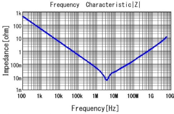
■ GRT188C80G475KE01 |Z| DCOV, 25degC
