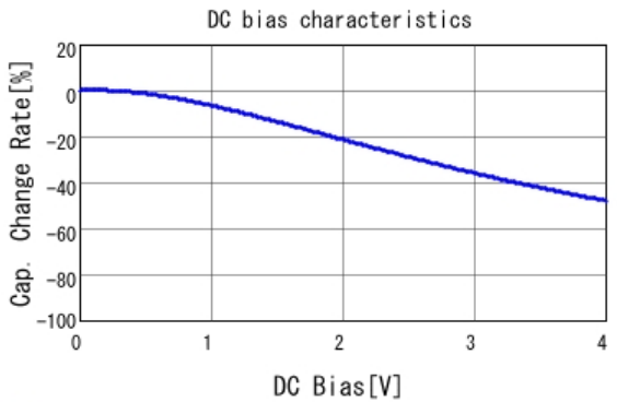
■ GRT188C80G475KE01 C-DC bias capchange, 25.0degC, AC0.
