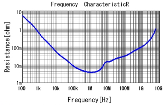
■ GRT188C80G475KE01 R DCOV, 25degC
