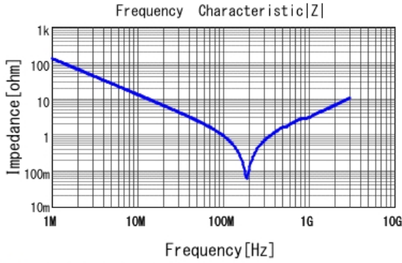
■ GRM21A7U2E122JW31 |Z| DCOV, 25degC
