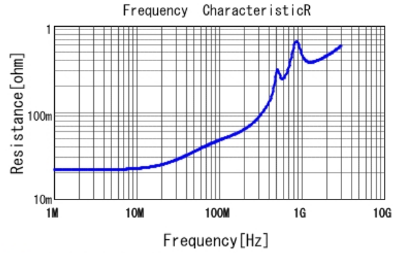
■ GRM21A7U2E122JW31 R DCOV, 25degC
