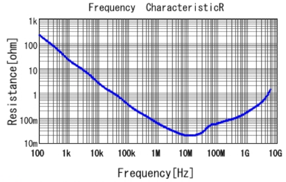
■ GRT155R61E224KE01 R DC0V, 25degC
