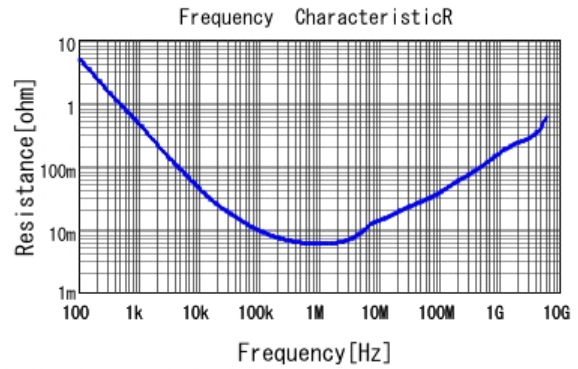
■ GRT155R60J475ME13 R DCOV, 25degC
