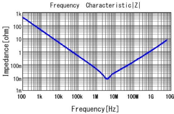
■ GRT155R60J475ME13 |Z| DCOV, 25degC
