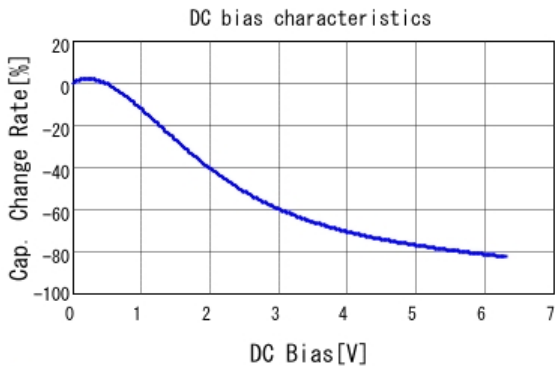
■ GRT155R60J475ME13 C-DC bias capchange, 25.0degC, ACO.
