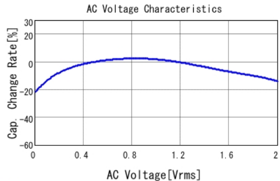
■ GRT155R60J475ME13 C-AC Voltage capchange, DCOV, 25.0d
