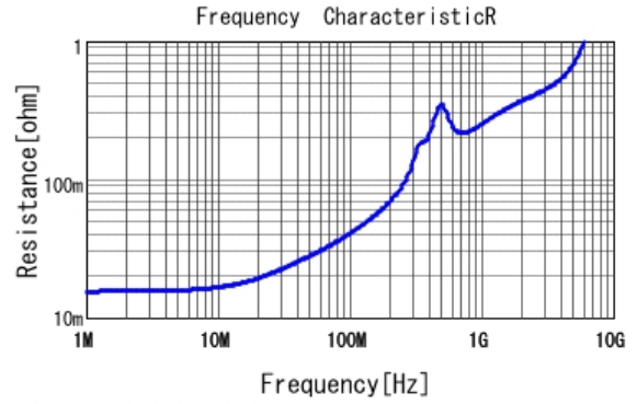
■ GRM1557U1A272JA01 R DCOV, 25degC
