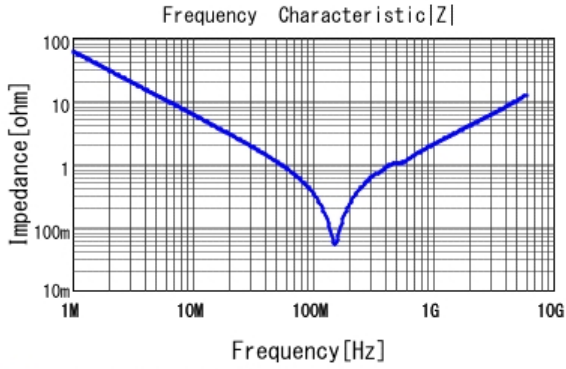
■ GRM1557U1A272JA01 |Z| DCOV, 25degC
