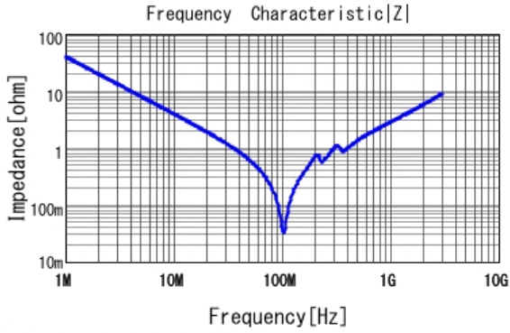
■ GRM21B7U2E392JW32 |Z| DCOV, 25degC
