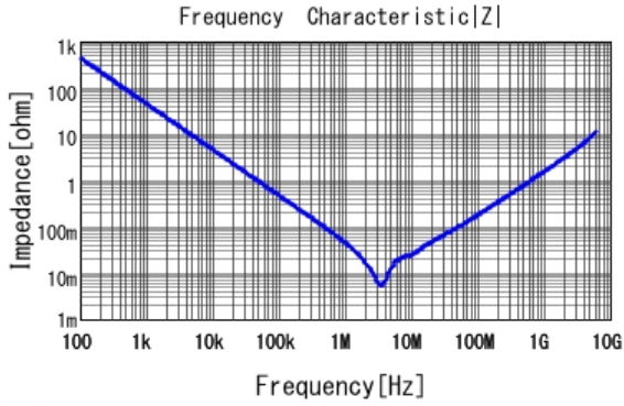
■ GRT188C81C475KE13 |Z| DCOV, 25degC
