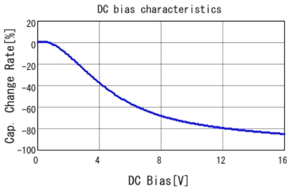
■ GRT188C81C475KE13 C-DC bias capchange, 25.0degC, AC1V
