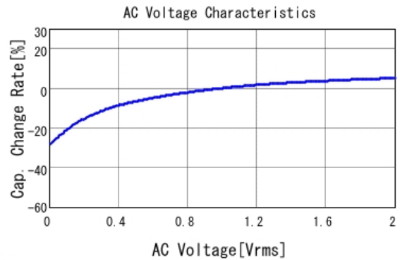
■ GRT188C81C475KE13 C-AC Voltage capchange, DCOV, 25.0d
