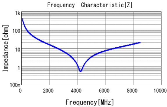
GCM1555C1H4R0CA16 |Z| DCOV, 25degC
