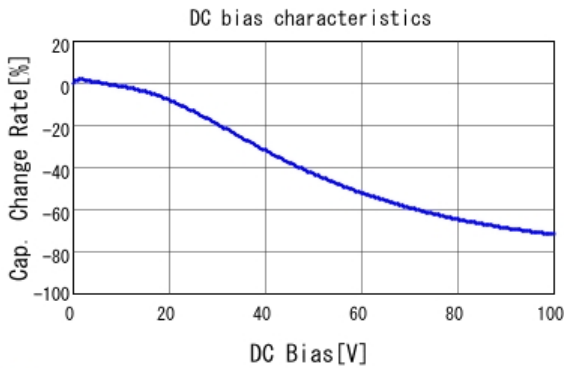
■ GRM155R72A472KA01 C-DC bias capchange, 25.0degC, AC1.
