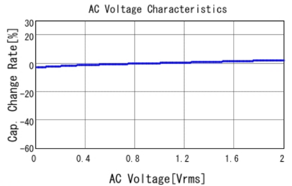
■ GRM155R72A472KA01 C-AC Voltage capchange, DCOV, 25.0d
