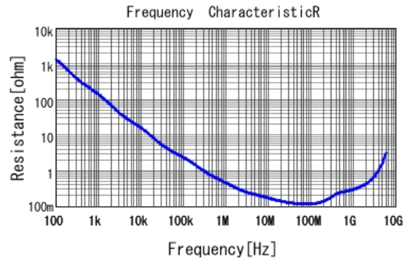
■ GRM155R72A472KA01 R DCOV, 25degC
