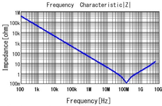
■ GRM155R72A472KA01 |Z| DCOV, 25degC
