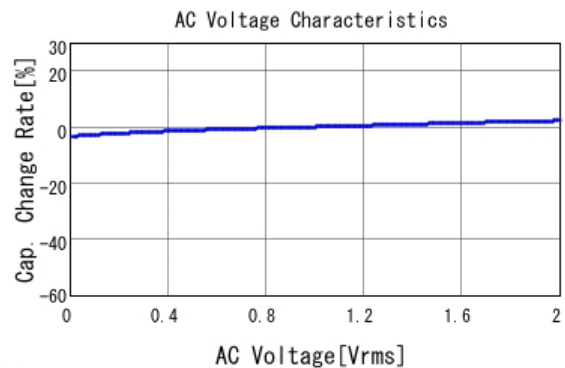
■ GCJ188R71E223KA01 C-AC Voltage capchange, DCOV, 25.0d
