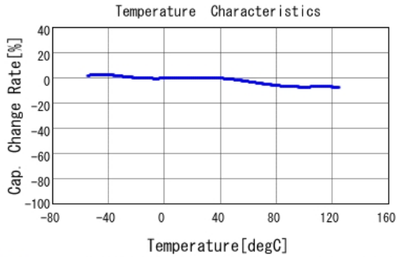
■ GCJ188R71E223KA01 C-Temp. capchange, DC0.0V, AC1.0Vrm
