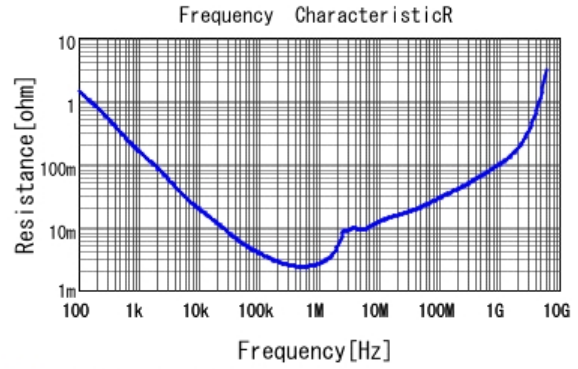
■ GRT21BR61C226ME13 R DCOV, 25degC
