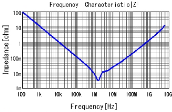
■ GRT21BR61C226ME13 |Z| DCOV, 25degC
