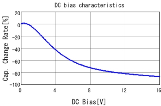
■ GRT21BR61C226ME13 C-DC bias capchange, 25.0degC, AC0.
