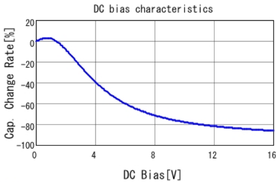
■ GRT155R61C474KE01 C-DC bias capchange, 25.0degC, AC1.
