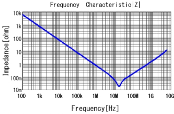
■ GRT155R61C474KE01 |Z| DC0V, 25degC
