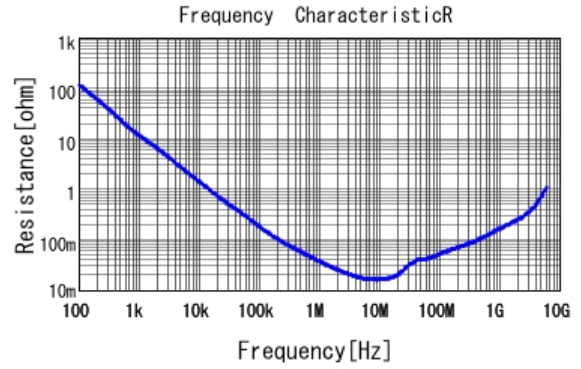
■ GRT155R61C474KE01 R DC0V, 25degC
