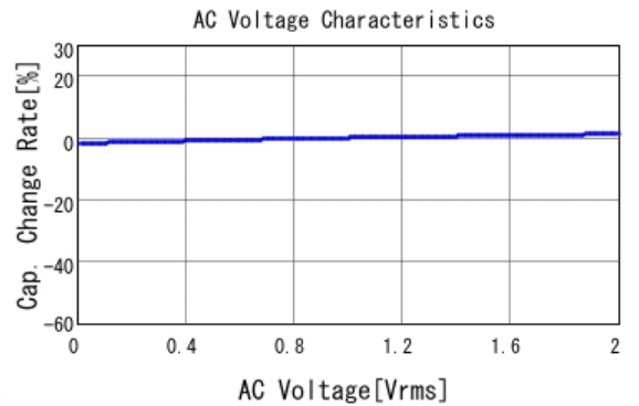
■ GCJ188R71H152KA01 C-AC Voltage capchange, DCOV, 25.0d
