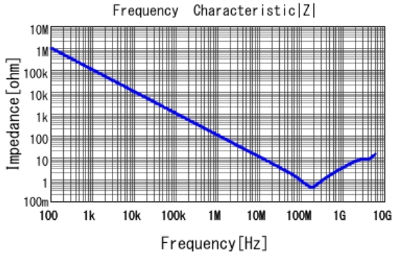
■ GCJ188R71H152KA01 |Z| DCOV, 25degC
