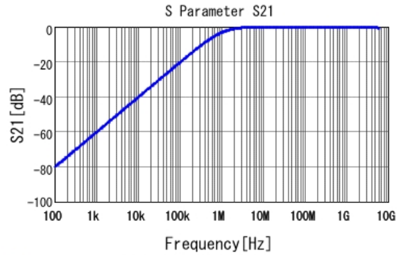
■ GCJ188R71H152KA01 S21 DC0V, 25degC
