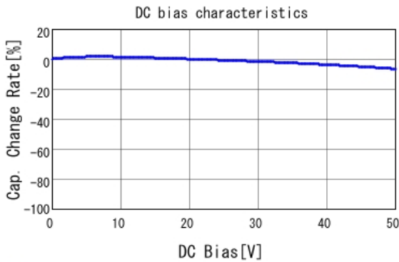
■ GCJ188R71H152KA01 C-DC bias capchange, 25.0degC, AC1.
