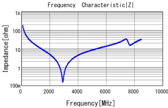
■ GJM1555C1H9R0CB01 |Z| DCOV, 25degC
