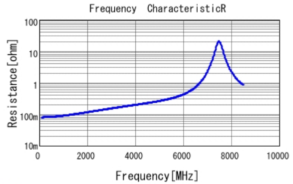
■ GJM1555C1H9R0CB01 R DCOV, 25degC
