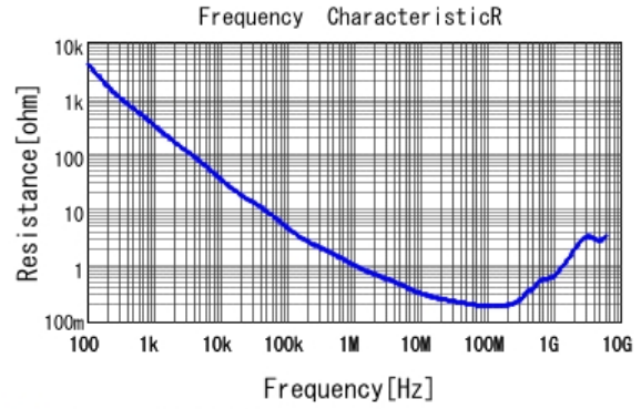
■ GCE188R72A222KA01 R DCOV, 25degC
