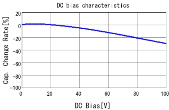
■ GCE188R72A222KA01 C-DC bias capchange, 25.0degC, AC1.
