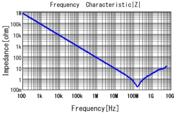
■ GCE188R72A222KA01 |Z| DCOV, 25degC
