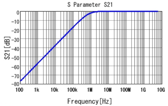
■ GCE188R72A222KA01 S21 DC0V, 25degC
