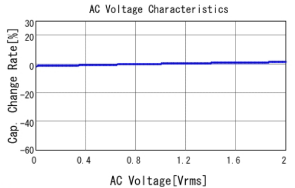
■ GCE188R72A222KA01 C-AC Voltage capchange, DCOV, 25.0d
