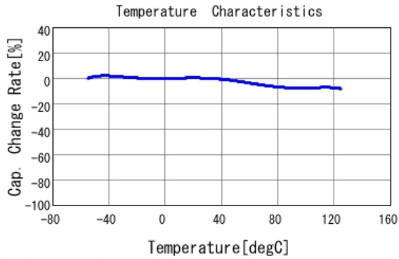
■ GCE188R72A222KA01 C-Temp. capchange, DC0.0V, AC1.0Vrm
