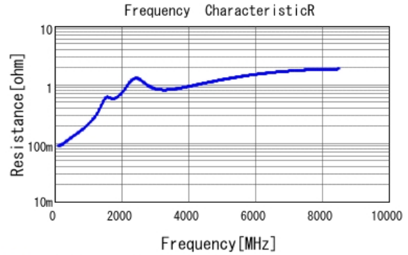
■ GCM1555C1H151JA16 R DCOV, 25degC
