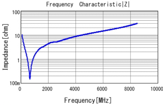
■ GCM1555C1H151JA16 |Z| DCOV, 25degC
