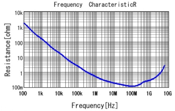
■ GRM155R71H472KA01 R DCOV, 25degC
