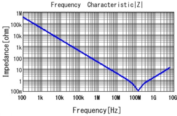
■ GRM155R71H472KA01 |Z| DCOV, 25degC
