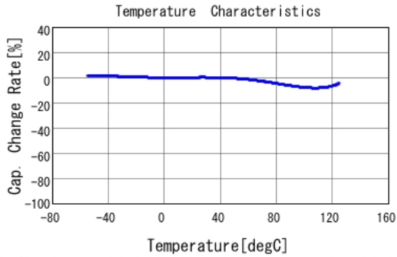
■ GCM155R72A681KA37 C-Temp. capchange, DC0.0V, AC1.0Vrm
