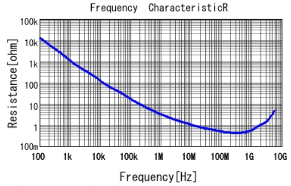
GCM155R72A681KA37 R DCOV, 25degC
