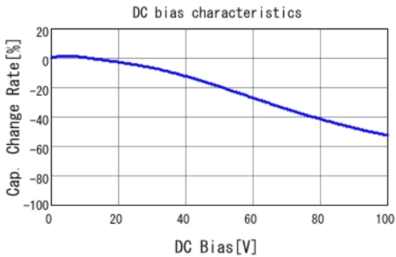
GCM155R72A681KA37 C-DC bias capchange, 25.0degC, AC1.
