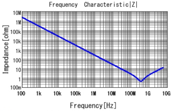
GCM155R72A681KA37 |Z| DCOV, 25degC
