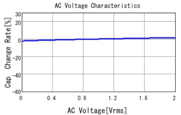
GCM155R72A681KA37 C-AC Voltage capchange, DCOV, 25.0d
