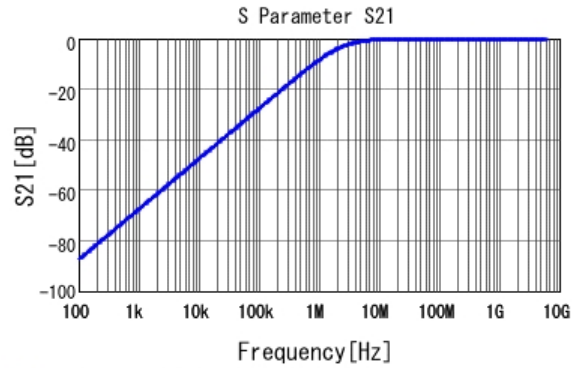
■ GCM155R72A681KA37 S21 DC0V, 25degC
