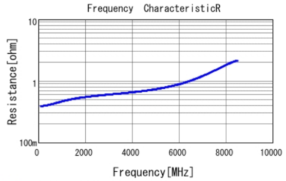
■ GCM1555C1H1R5WA16 R DCOV, 25degC
