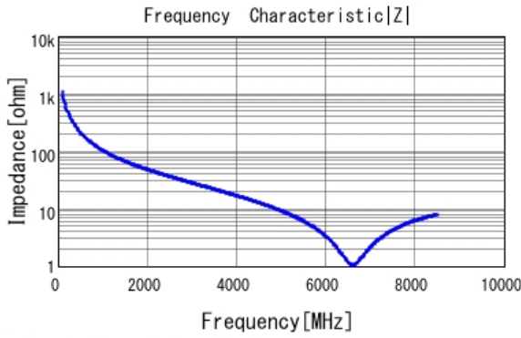
■ GCM1555C1H1R5WA16 |Z| DCOV, 25degC
