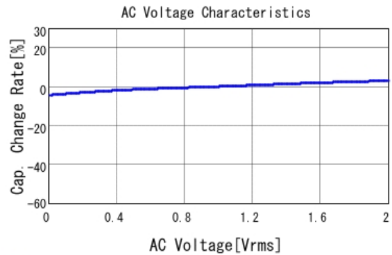
GCM155R71C473KA37 C-AC Voltage capchange, DCOV, 25.0d
