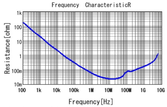
GCM155R71C473KA37 R DCOV, 25degC
