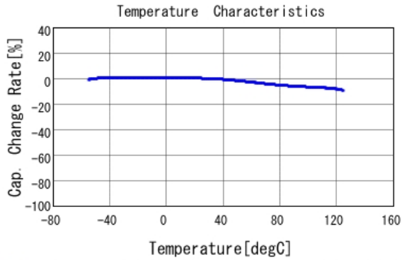
■ GCM155R71C473KA37 C-Temp. capchange, DC0.0V, AC1.0V rm
