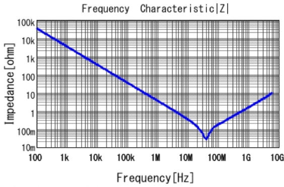
GCM155R71C473KA37 |Z| DCOV, 25degC
