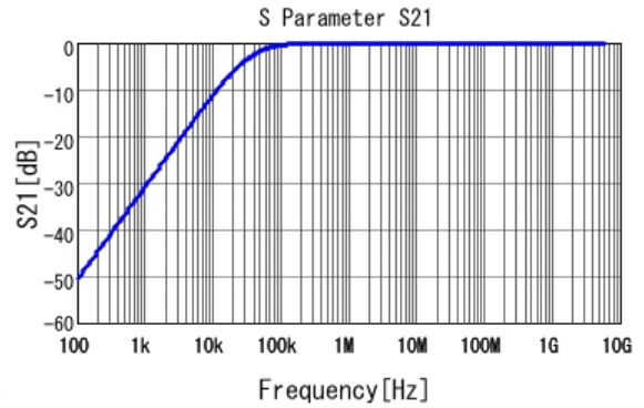
■ GCM155R71C473KA37 S21 DC0V, 25degC
