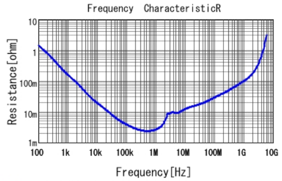
■ GRM21BC81A226ME44 R DCOV, 25degC
