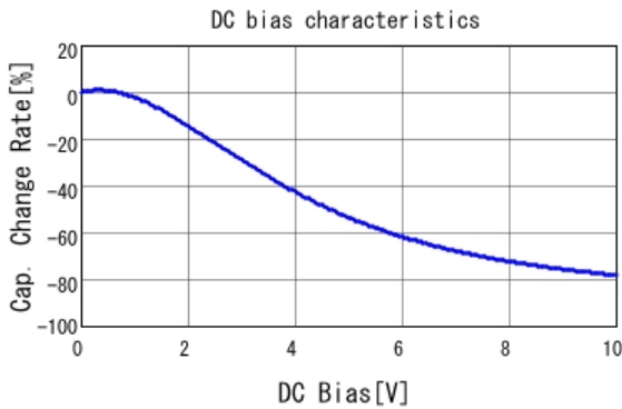
■ GRM21BC81A226ME44 C-DC bias capchange, 25.0degC, AC0.
