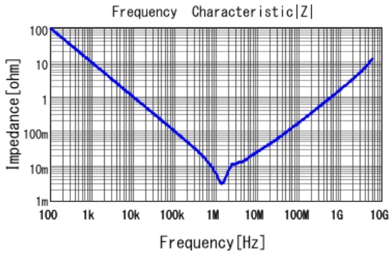
■ GRM21BC81A226ME44 |Z| DCOV, 25degC
