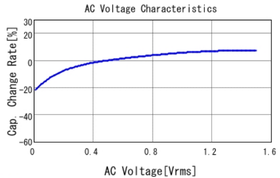
■ GRM21BC81A226ME44 C-AC Voltage capchange, DCOV, 25.0d
