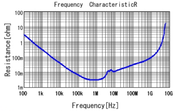
■ GRM21BC71E106ME11 R DCOV, 25degC
