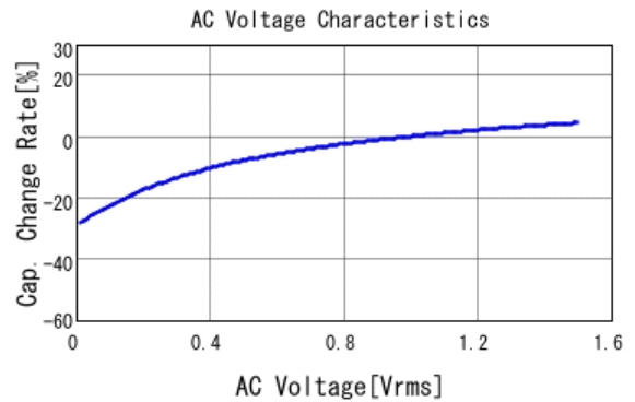
■ GRM21BC71E106ME11 C-AC Voltage capchange, DCOV, 25.0d
