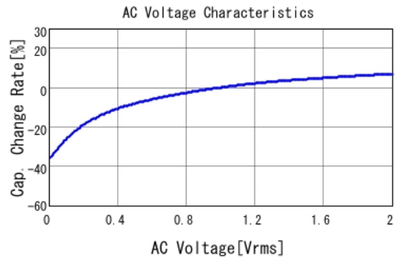
■ GRM188R61E225KA12 C-AC Voltage capchange, DCOV, 25.0d
