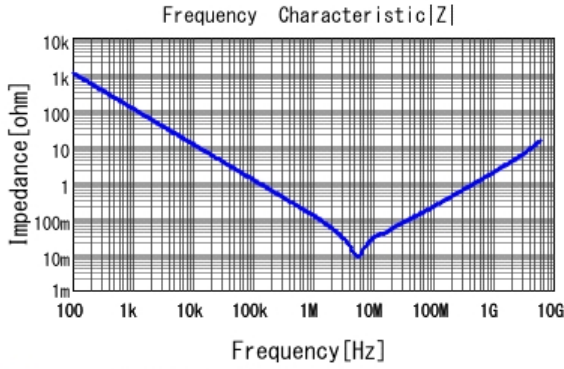
■ GRM188R61E225KA12 |Z| DCOV, 25degC
