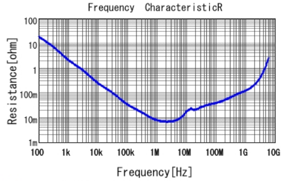
■ GRM188R61E225KA12 R DCOV, 25degC
