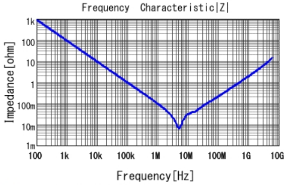
■ GRM188R61H225KE11 |Z| DCOV, 25degC
