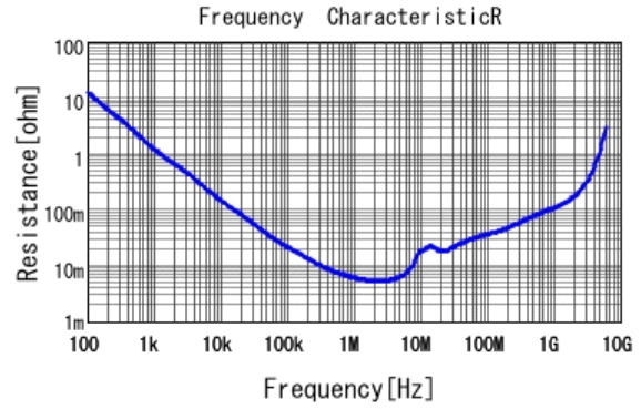
■ GRM188R61H225KE11 R DCOV, 25degC
