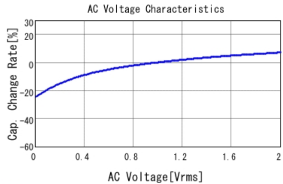
■ GRM188R61H225KE11 C-AC Voltage capchange, DCOV, 25.0d
