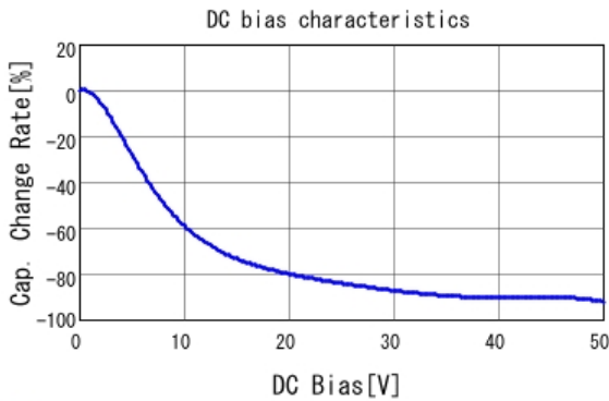
■ GRM188R61H225KE11 C-DC bias capchange, 25.0degC, AC1V
